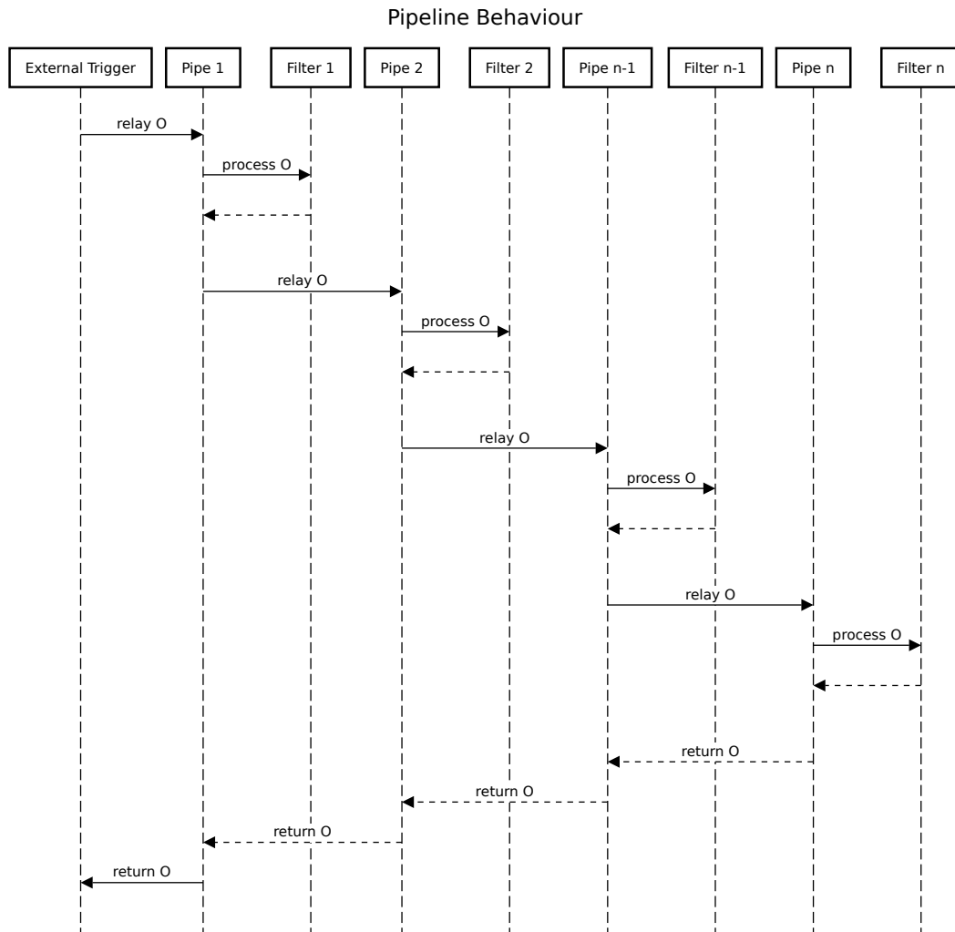
Figure 3.1.: An abstract sequence diagram of the pipes and filters design pattern. The relaying mechanism used by pipes in this diagram is realized through method calls.
